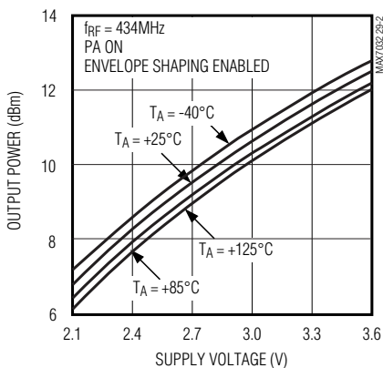
OUTPUT POWER vs. SUPPLY VOLTAGE MAX7032 29-2
